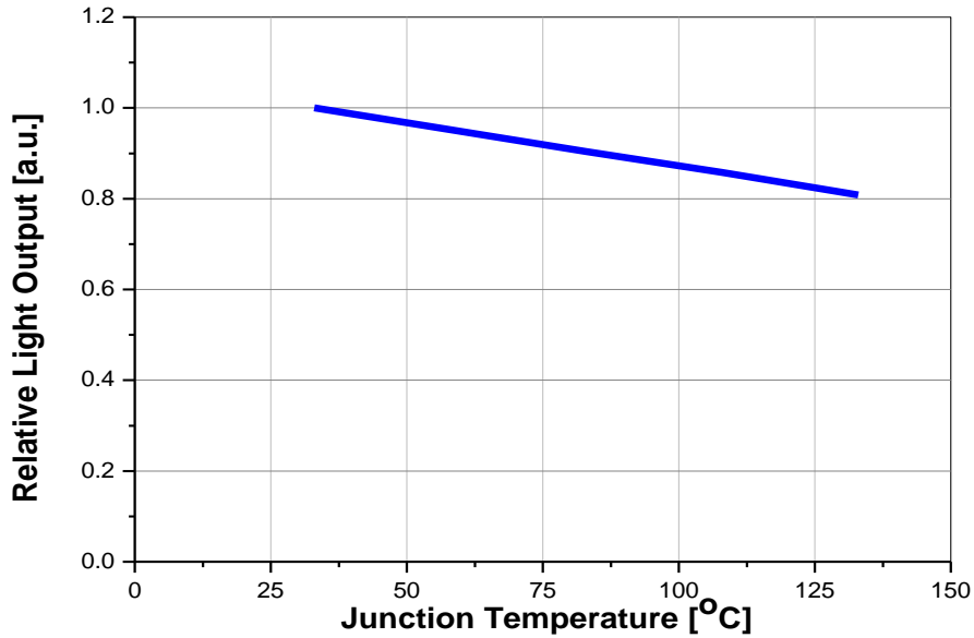
Fig 6. Relative Light Output vs. Junction Temperature, I_F=20\text{mA}
